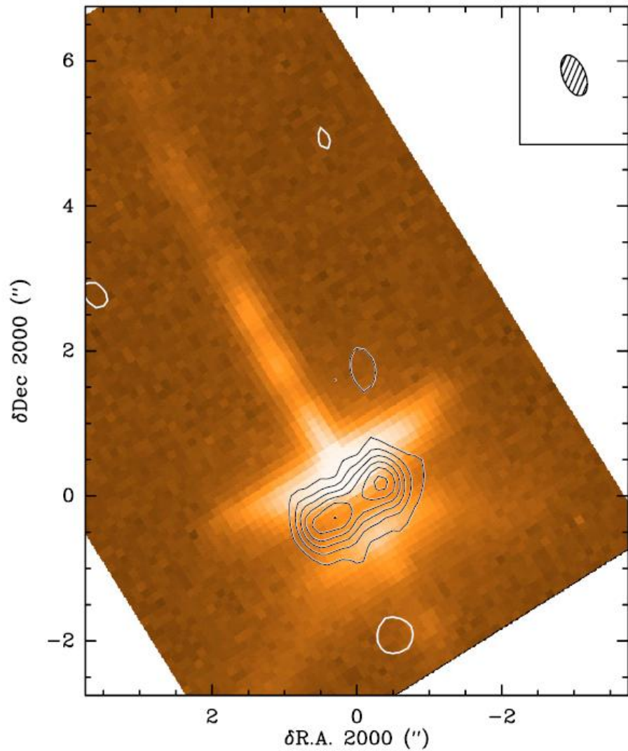
Disc seen directly in molecular gas (CO) (contours) perpendicular to jet
